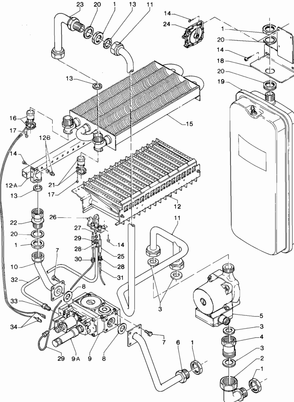
COMPONENTI INTERNI A - INTERNAL COMPONENTS A
