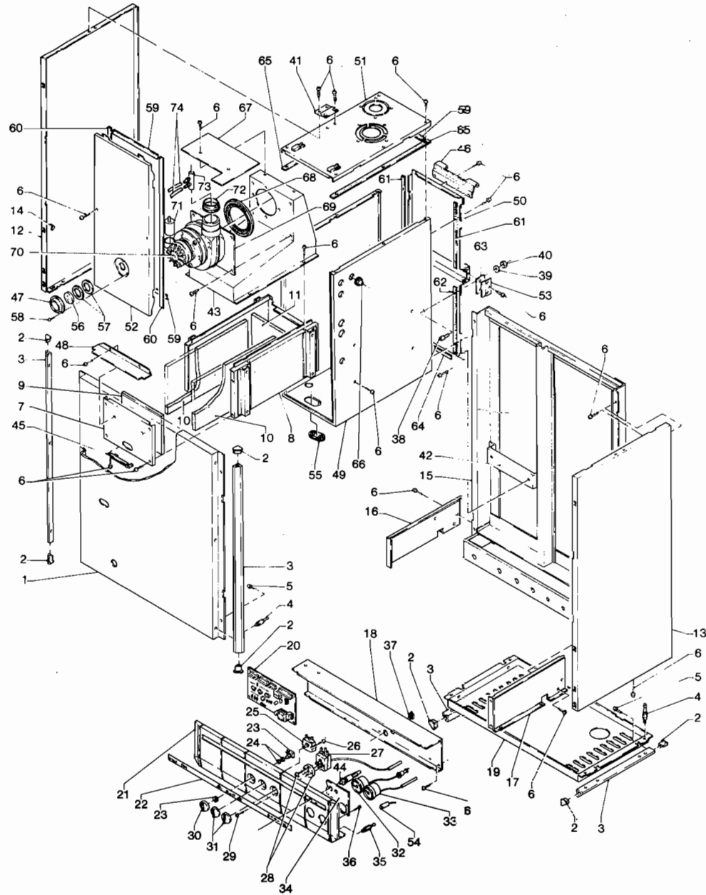
MANTELLO - OUTSIDE PANEL
