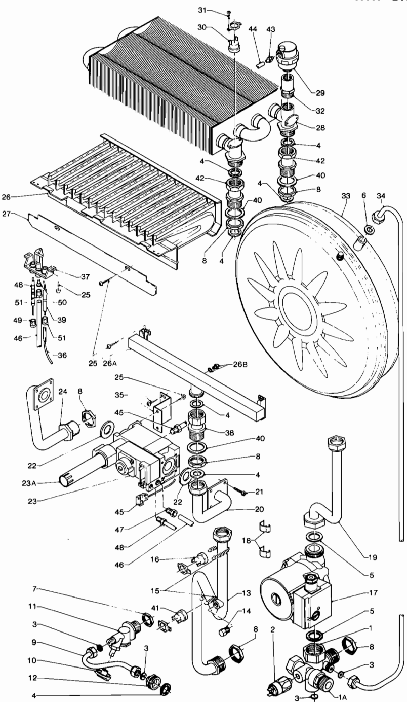
COMPONENTI INTERNI - INTERNAL COMPONENTS
