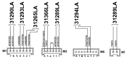
SCHEMA BMBC c/DISPLAY DIGITECH - SM20019 COD. 76677LA
