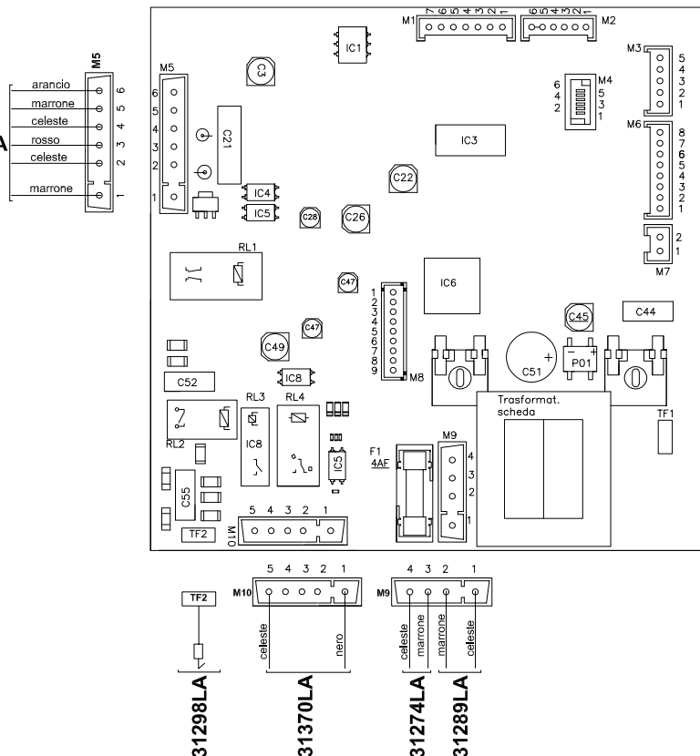
SCHEMA BMBC c/DISPLAY DIGITECH - SM20019 COD. 76677LA
