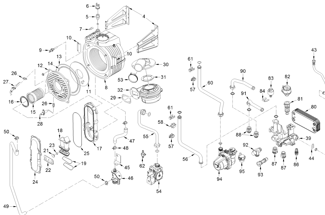
BRAVA DGT HE 12 T - interno
